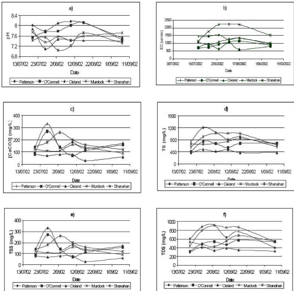
Figure 2.2: Szymanski and Patterson (2003) - Analysis of water quality parameters (a) pH b) EC c) Alkalinity d) Total solids e) Total suspended solids f) Total dissolved solids) in septic tanks injected with EM
