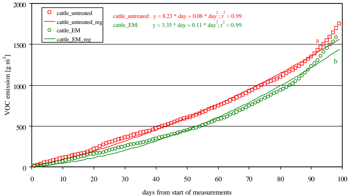
Figure 16 Cumulated VOC emissions from cattle slurry with and without addition of EM.
